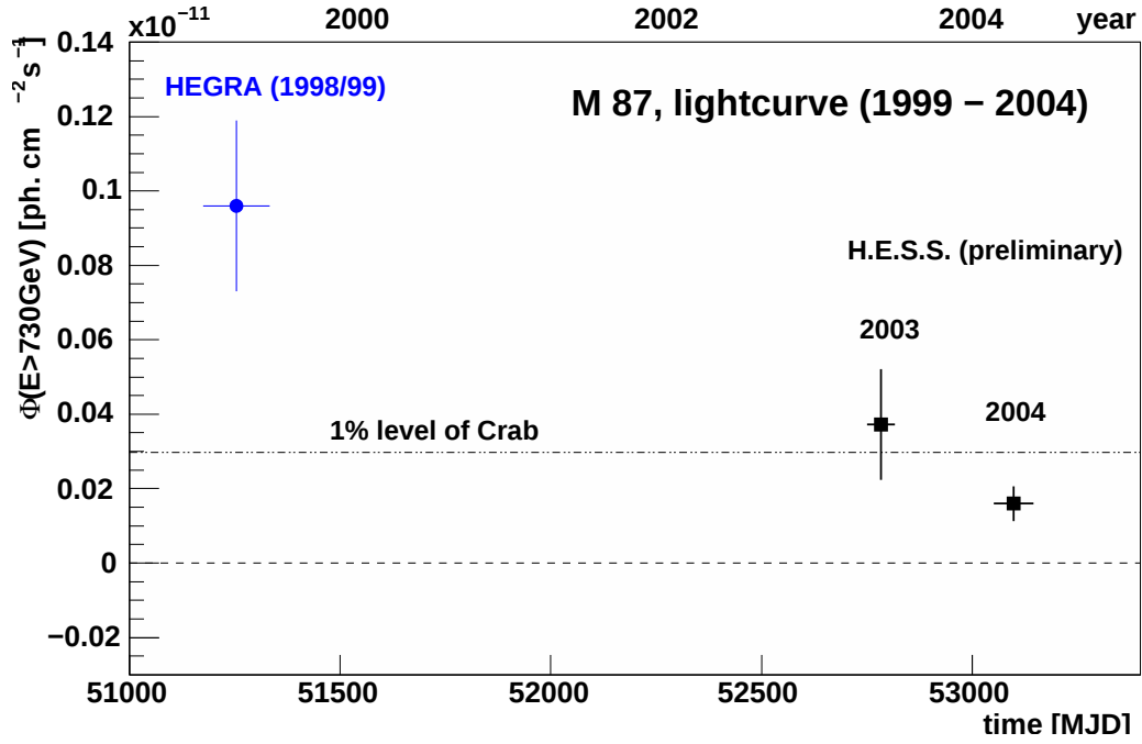
FIG. 5: The integral photon flux above an threshold of 730 GeV is shown. The recent H.E.S.S. measurement in 2004 is clearly not compatible with the HEGRA flux (taken from [9]) which indicates variability. The 1 % flux level of the Crab Nebula is also indicated underlining the very low (but significant) flux of M 87 in 2004.
