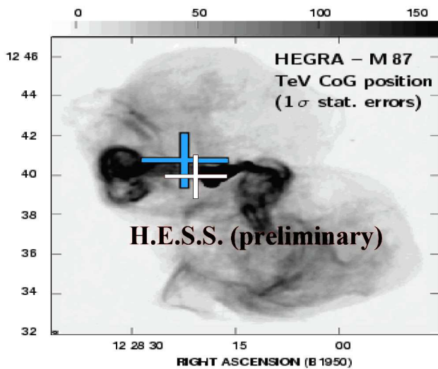
FIG. 4: The positions of the H.E.S.S. TeV excess (white cross) together with the position measured by HEGRA (filled cross) plotted in the radio map of M 87 (adopted from [19]). Within statistical errors, both positions are compatible with the M 87 central region.
