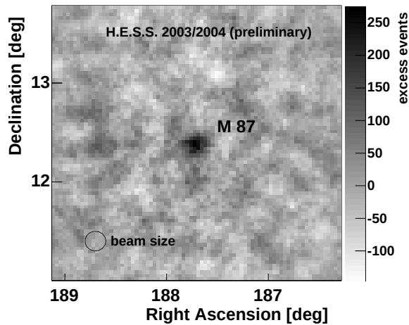
FIG. 3: The TeV excess sky map showing a 3^\circ \times 3^\circ sky region centered around the position of M 87. The number of events are integrated within the optimal point-source angular cut of \Theta \leq 0.11^\circ for each of the correlated bins. The background is estimated using the ring background model. The event-by-event angular resolution is indicated by the circle (beamsize).
