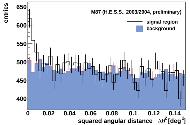
FIG. 2: Distribution of ON-source events (solid histogram) and normalized OFF-source events (filled histogram) vs. the squared angular distance \Delta\Theta^2 between the reconstructed shower direction and the nominal object position.
