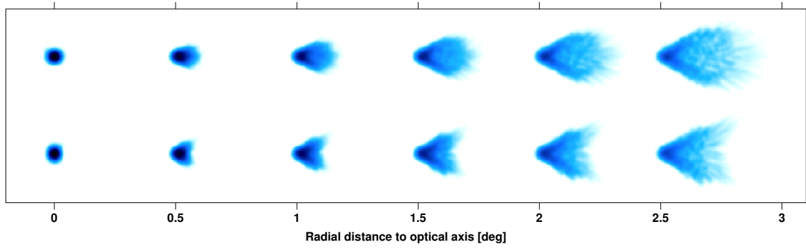
Figure 3. Simulated point spread function of the H.E.S.S. II reflector for various angular distances to the optical axis. The top series of shapes represent the (rotated) evolution in the vertical direction; the bottom series are for the horizontal direction. The intensity scale is logarithmic. Note that the actual active field of view is limited to a radius of 1.6 degrees.
